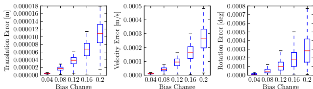
Fig. 11: Error committed when using the first-order approximation (44) instead of repeating the integration, for different bias perturbations. Left: \Delta \hat{\mathbf{p}}_{ij}(\mathbf{b}_i + \delta \mathbf{b}_i) error; Center: \Delta \hat{\mathbf{v}}_{ij}(\mathbf{b}_i + \delta \mathbf{b}_i) error; Right: \Delta \hat{\mathbf{r}}_{ij}(\mathbf{b}_i + \delta \mathbf{b}_i) error. Statistics are computed over 1000 Monte Carlo runs.
