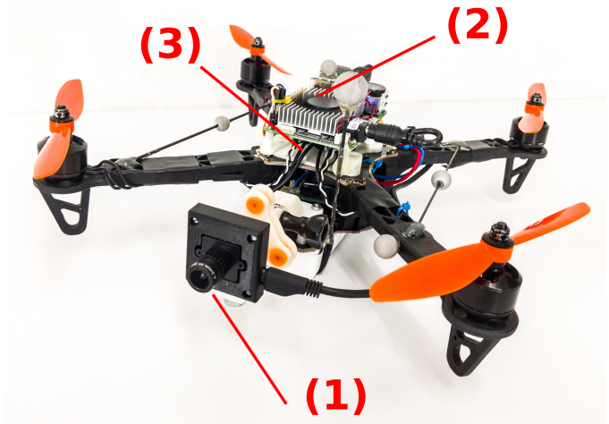
Fig. 8: The quadrotor used for the experiments. (1) The Insignthness SEEM1 sensor. (2) The Intel Upboard computer, running the detection algorithm. (3) The Lumenier F4 AIO flight controller, receiving commands from the ground station.
