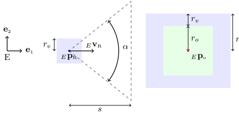
Fig. 1: A schematics representing the obstacle and the robot model in the frame E . The robot is represented as a square of size 2r_v centered at {}^E P_R , and moves with a speed {}^E V_R . The dashed triangle starting from the robot's position represents its sensing area, \alpha is the field of view and s the maximum distance it is able to perceive. The obstacle, represented by the green square on the right side of the image, has size 2r_o . We expand the square representing the obstacle by a quantity r_v such that the robot can be considered to be a point mass.
