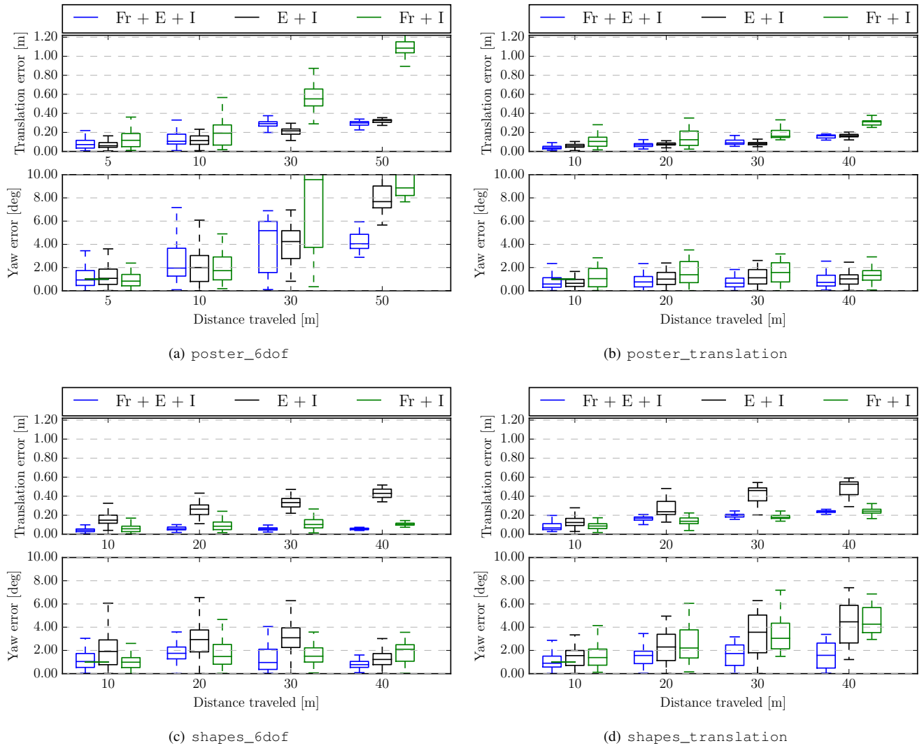
Fig. 9. (Continuation) Detailed comparison of the pipeline performance on the Event Camera Dataset, while using standard frames (Fr), events (E), and IMU (I); events and IMU; and images and IMU.
