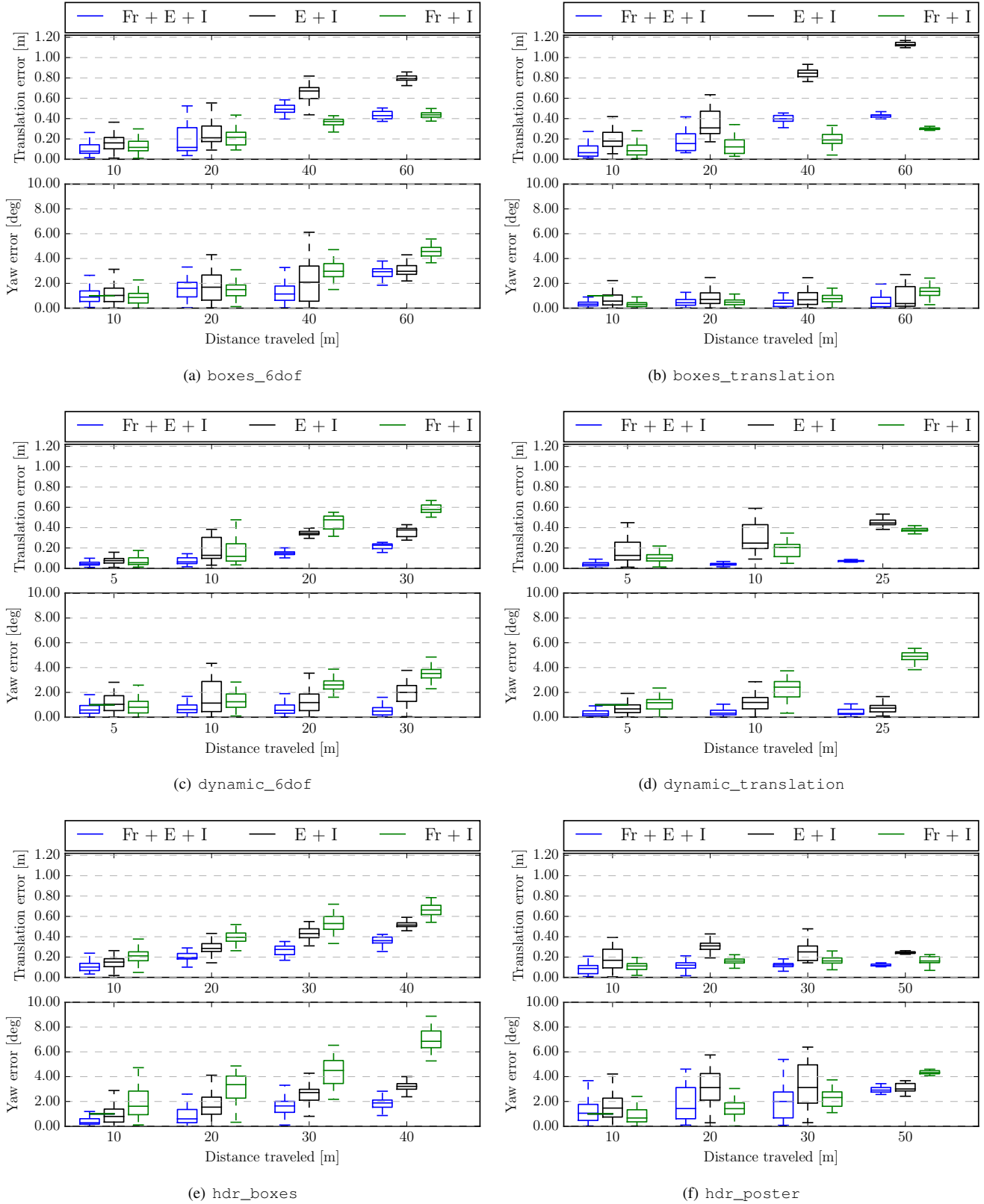
Fig. 8. Detailed comparison of the pipeline performance on the Event Camera Dataset, while using standard frames (Fr), events (E), and IMU (I); events and IMU; and images and IMU.
