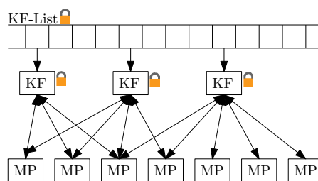
Figure A.3 – Data-structure design for concurrency.
