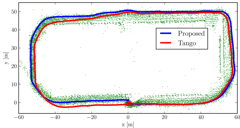
Figure C.18 – Outdoor trajectory (length: 300m) around a building with identical start and end point at coordinates (0,0,0) . The end-to-end error of the proposed approach is 1.0m. Google Tango accumulated 2.2m drift. The green dots are the 3D points triangulated from our trajectory estimate.
