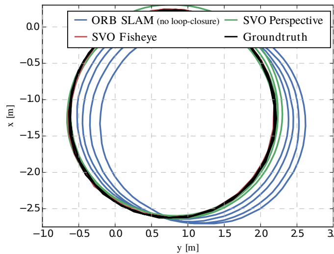
Figure B.18 – Comparison of perspective and fisheye lens on the same circular trajectory that was recorded with a micro aerial vehicle in a motion capture room. The ORB-SLAM result was obtained with the perspective camera images and loop-closure was deactivated for a fair comparison with SVO. ORB-SLAM with a perspective camera and with loop-closure activated performs as good as SVO with a fisheye camera.
