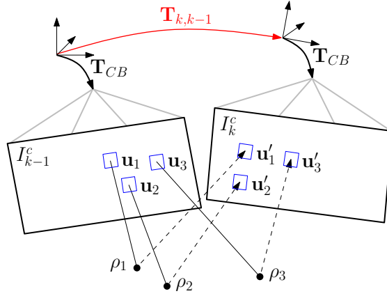
Figure B.2 – Changing the relative pose T_{k,k-1} between the current and the previous frame implicitly moves the position of the reprojected points in the new image u'_i . Sparse image alignment seeks to find T_{k,k-1} that minimizes the photometric difference between image patches corresponding to the same 3D point (blue squares). Note, in all figures, the parameters to optimize are drawn in red and the optimization cost is highlighted in blue.
