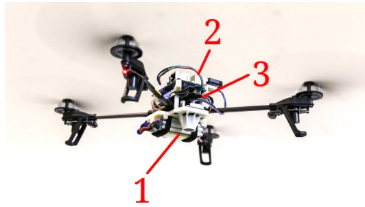
Figure E.7 – Experimental platform with (1) down-looking camera, (2) on-board computer, and (3) inertial measurement unit.
