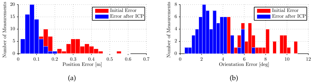
Figure F.11 – (a) Distribution of the translation error before and after ICP pose refinement. The data originates from 67 experiments in 3 different environments. The median error is 0.076 m. (b) Distribution of the angular error before and after ICP pose refinement. The provided angle derives from the angle-axis representation of the orientation error. The data originates from 67 experiments. The median error is 3.0 deg.
