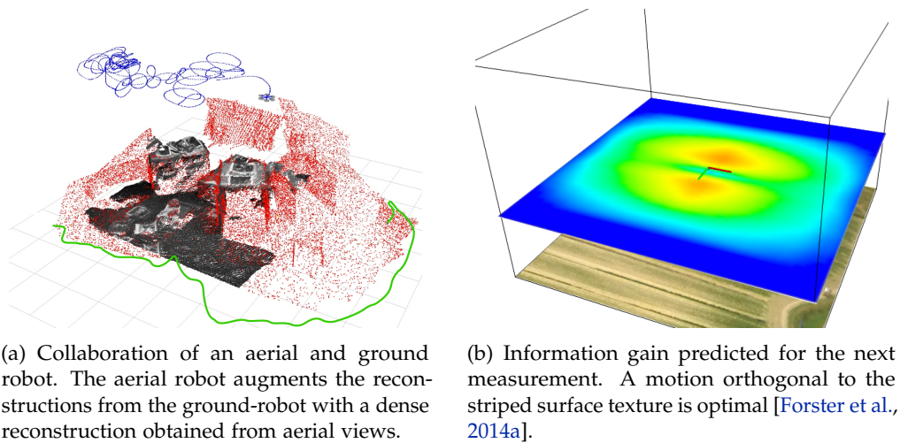
Figure 2.4 – Application of dense reconstruction for MAVs.
