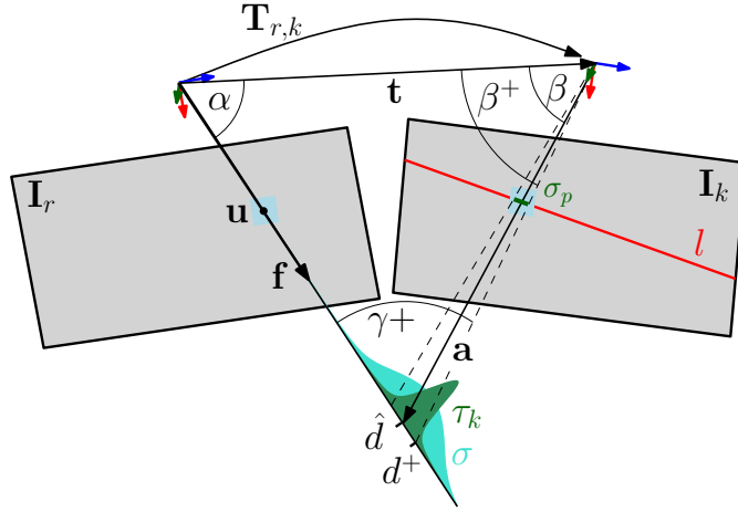
Figure G.2 – The uncertainty in depth measurement, \tau_k^2 , is computed by projecting the disparity uncertainty \sigma_p in image I_k on the pixel bearing-vector f .
