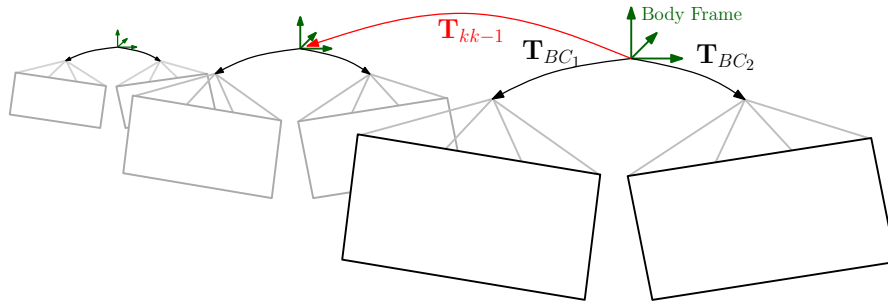
Figure B.9 – Visual odometry with multiple rigidly attached and synchronized cameras. We know the relative pose of each camera to the body frame T_{BC_j} from extrinsic calibration and the goal is to estimate the relative motion of the body frame T_{kk-1} .
