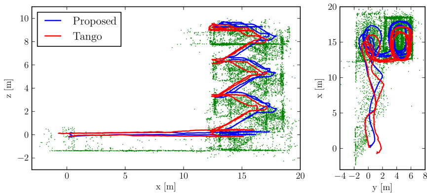
Figure C.19 – Real test comparing the proposed VIN approach against Google Tango. The 160m-long trajectory starts at (0,0,0) (ground floor), goes up till the 3rd floor of a building, and returns to the initial point. The figure shows a side view (left) and a top view (right) of the trajectory estimates for our approach (blue) and Tango (red). Google Tango accumulates 1.4m error, while the proposed approach only has 0.5m drift. 3D points triangulated from our trajectory estimate are shown in green for visualization purposes.
