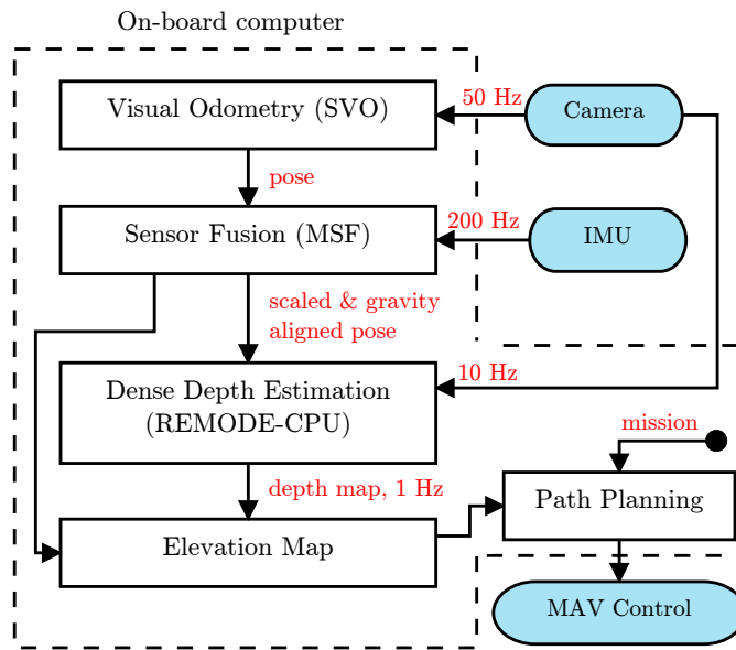
Figure E.2 – Overview of the main components and connections in the proposed system. All modules are running on-board the MAV.
