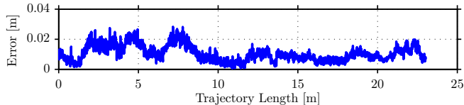
Fig. 9: Translation error of the Monocular SLAM on the MAV. The trajectory is 23.0 meters long and the RMS error is 1.2 cm. There is no visible drift because the trajectory contains many loops.
