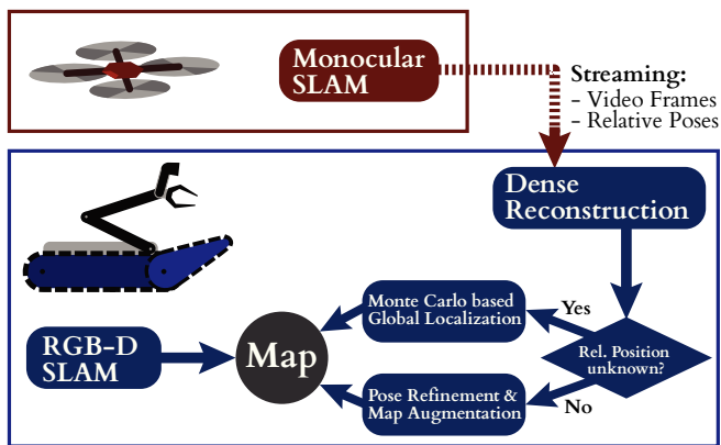
Fig. 4: Illustration of the localization and mapping pipeline. Each building block is described in detail in Sections IV to VII.
