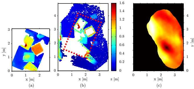
Fig. 7: The height maps of an aerial and a ground-based map are illustrated in Figures (a) and (b) respectively. The red dotted square in (b) shows the best alignment of the two height-maps. The costmap in (c) illustrates the ZMSSD cost for every possible relative position \mathbf{u} of the two maps. A global minima is located at the dark spot.
