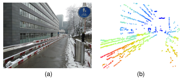
Figure 7. Example of monocular depth estimation with a hand-held event camera. (a) Scene, (b) semi-dense depth map, pseudo-colored from red (close) to blue (far). Image courtesy of [19].
