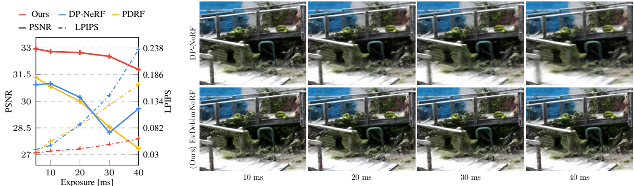
Figure 8. Robustness to motion blur analysis on the factory sample of Ev-DeblurBlender (left). Figures on the right show a qualitative comparison between DP-NeRF and Ev-DeblurNeRF among different exposures.
