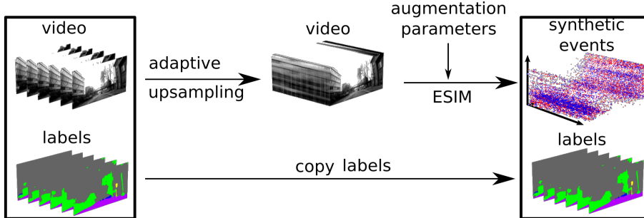
Figure 2. Overview of the method. Low frame-rate video is first adaptively upsampled using the method proposed in [17]. This upsampled video is fed to the event camera simulator (ESIM) [32] which produces asynchronous and sparse events with high temporal resolution.
