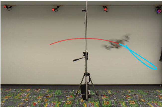
Fig. 7: Our quadrotor executing the whole trajectory split into approach (blue), traverse (red). In background the motion-capture system used to record the ground truth.
