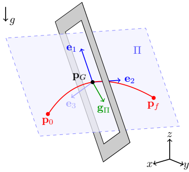
Fig. 2: An inclined gap and the corresponding plane II.
