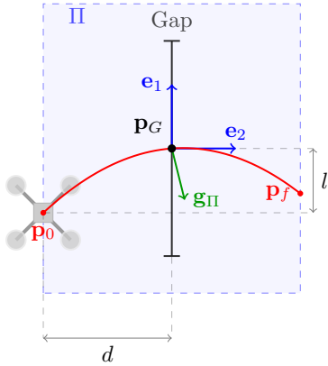
Fig. 3: The traverse trajectory in the plane II.
